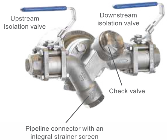
STS17.2 up to 17.5 bar g Steam trapping station
